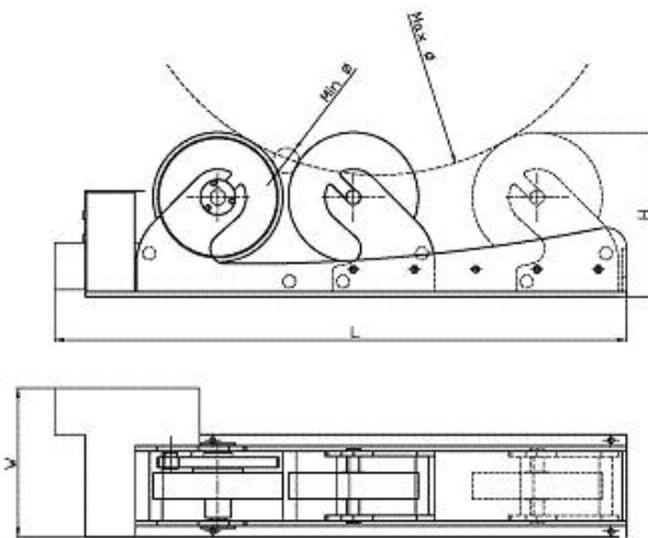
Drive unit
