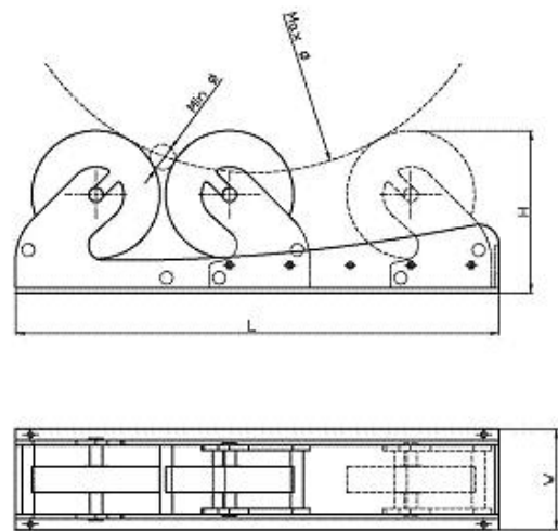
Idler unit
